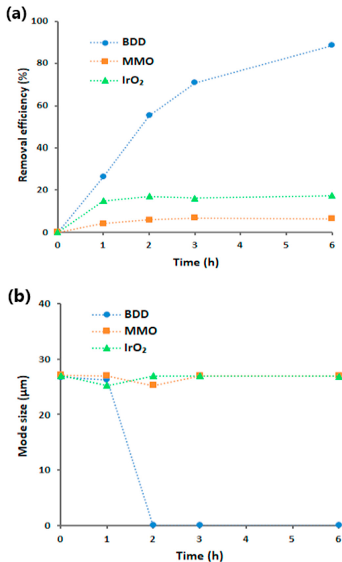
Fig. 4. The effect of anode material on the EO of MPs. (a) Removal efficiency (%), (b) Mode size (µm).
