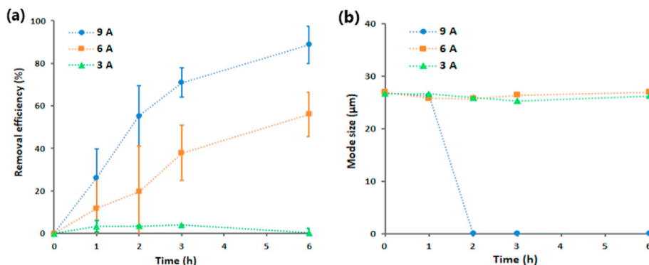
Fig. 2. The effect of current density on the EO of MPs. (a) Removal efficiency (%), (b) Mode size (μm).
