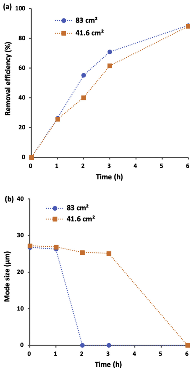
Fig. 3. The effect of anode surface area on the EO of MPs. (a) Removal efficiency (%), (b) Mode size (µm).
