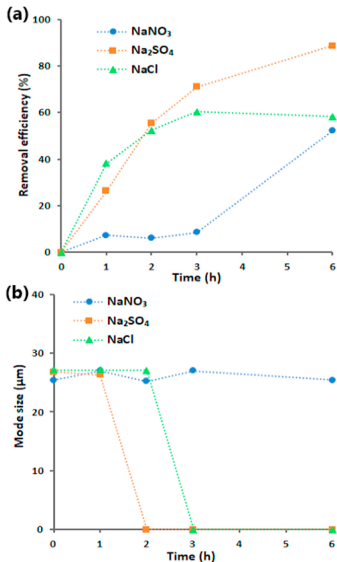
Fig. 5. The effect of electrolyte type on the EO of MPs. (a) Removal efficiency (%), (b) Mode size (μm).
