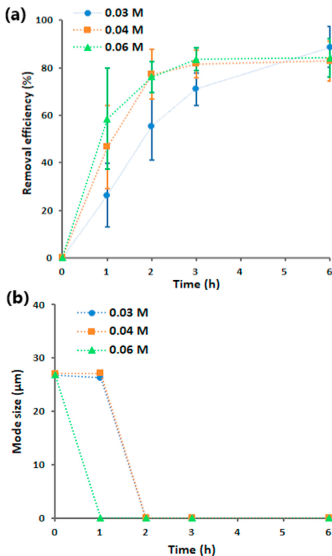
Fig. 6. The effect of electrolyte concentration on the EO of MPs. (a) Removal efficiency (%), (b) Mode size (μm).
