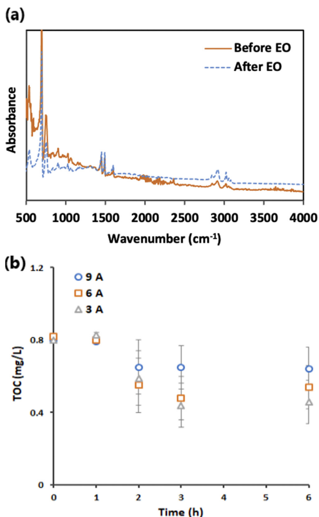
Fig. 8. (a) FTIR spectra of MPs before and after 1 h of EO, (b) TOC analysis of filtered treated water at different current intensities.
